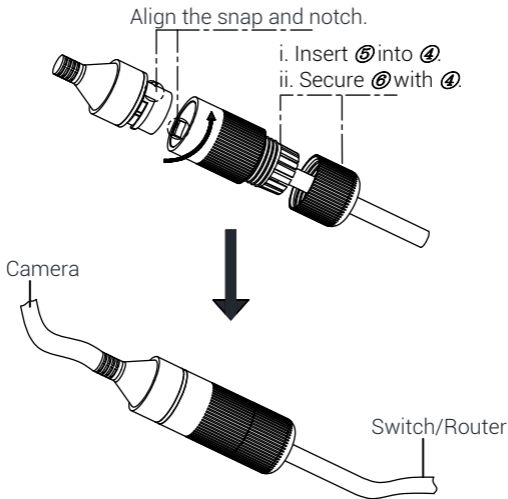
Figure 2-13 Water-proof Accessory Installation
